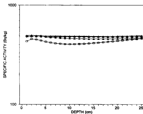
Fig 1. Vertical distribution of ^{40}\text{K} at studied locations. —▲—: Četekovac; —■—: G Polje; —□—: Pokupsko; —○—: Daruvar; —○—: Zagreb.
