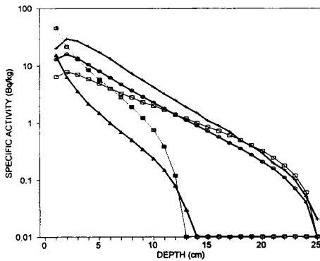
Fig 2. Vertical distribution of ^{134}\text{Cs} at studied locations. —▲—: Četkovac; —■—: G Polje; —□—: Pokupsko; —○—: Daruvar; —○—: Zagreb.
