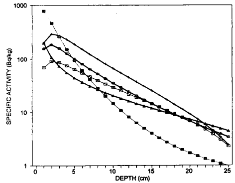
Fig 3. Vertical distribution of ^{137}\text{Cs} at studied locations. —▲—: Četkovac; —■—: G Polje; —□—: Pokupsko; —○—: Daruvar; —○—: Zagreb.
