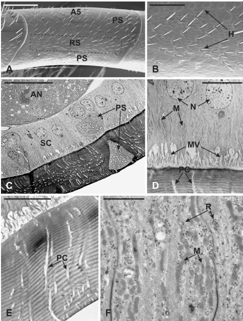
Figure 1. SEM micrographs of Apis mellifera drone 5th antennomere (A5) showing (in A) the release site of the glands (as shown inside the dashed rectangular box) surrounded by the plate sensilla and (in B) detail of the cuticle with evidence of the non-innervated hairs. TEM micrographs of A5 cross sections showing the thick glandular epithelium appressed to the cuticle (in C), details of the secretory cells (in D), particulars of the cuticle with the pore canals (in E) and cytological features of the secretory cells (in F). AN, antennal nerve; H, non-innervated hairs; M, mitochondria; MV, microvilli; N, nuclei; PC, pore canals; PS, plate sensilla; R, ribosomes; RS, release site; SC, secretory cells. Bar scale: A = 100 \mu\text{m} , B = 50 \mu\text{m} , C = 20 \mu\text{m} , D = 5 \mu\text{m} , E = 10 \mu\text{m} , F = 1 \mu\text{m} .
